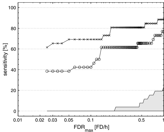
Fig. 5. Performance of the seizure detection method with respect to FDR_{max} obtained from scalp EEG ( \times ) and from invasive EEG ( \circ ) recordings. Gray shaded areas mark regions below averaged critical values \sigma_{rand,0.05} of a 5% significance level of a random detector.
