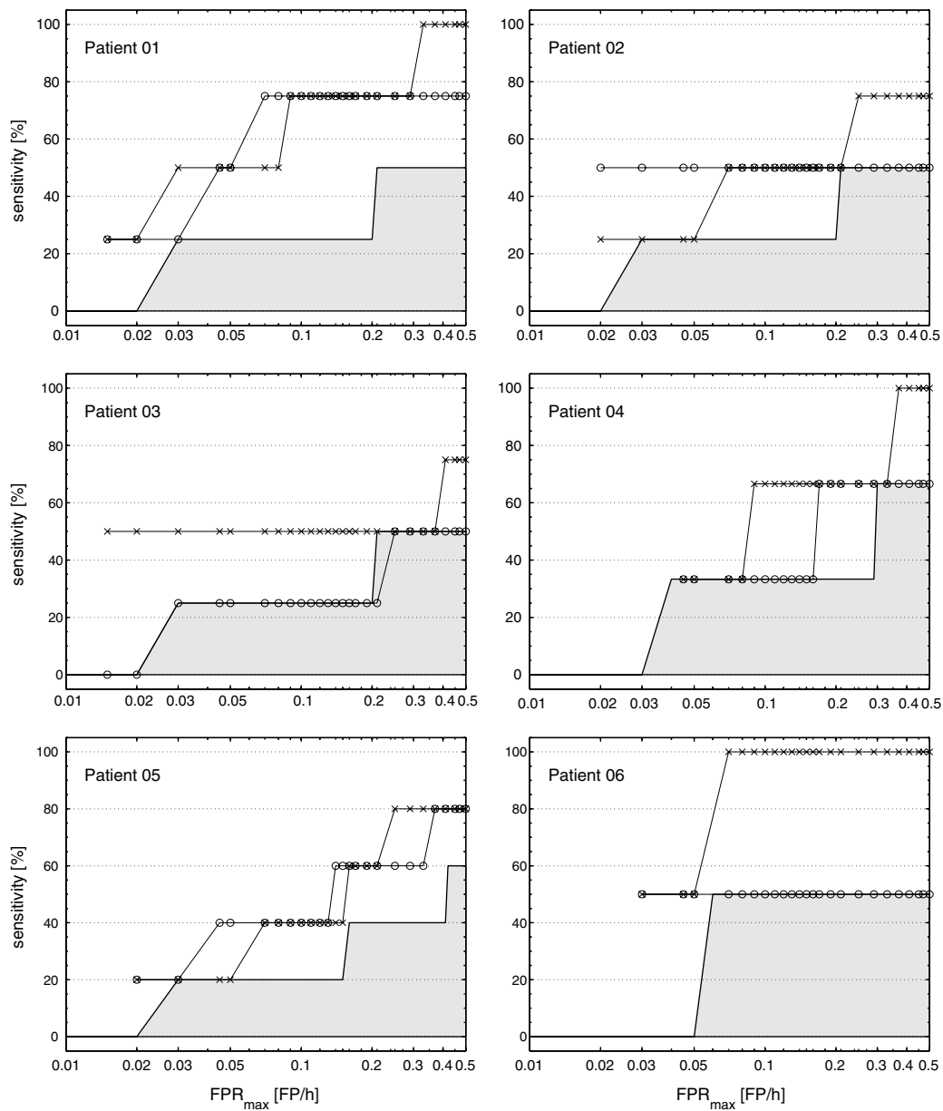
Fig. 8. Sensitivity of the investigated seizure prediction method in dependence on maximum false prediction rate for each patient. IT and SOP are fixed at 5 and 30 min, respectively. Different graphs result from scalp EEG (x) and from invasive EEG (o) recordings. Gray shaded areas mark regions below critical values \sigma_{rand,0.05} of a 5% significance level of a random predictor.
