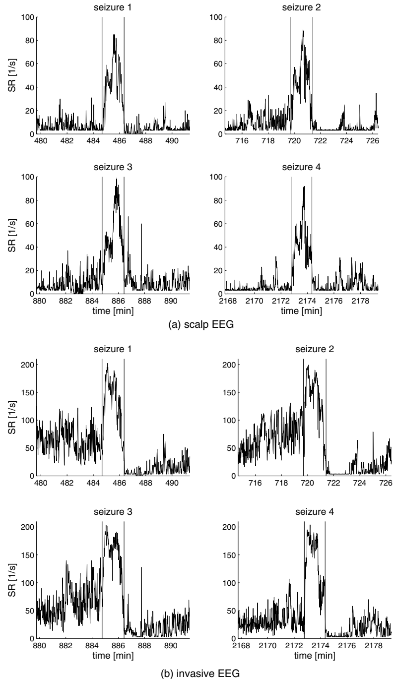
Fig. 2. Extractions of the spiking rate from scalp (a) and invasive (b) EEG data at four seizures of patient 01. The electroencephalographic seizure onsets and seizure ends are marked by vertical lines.
