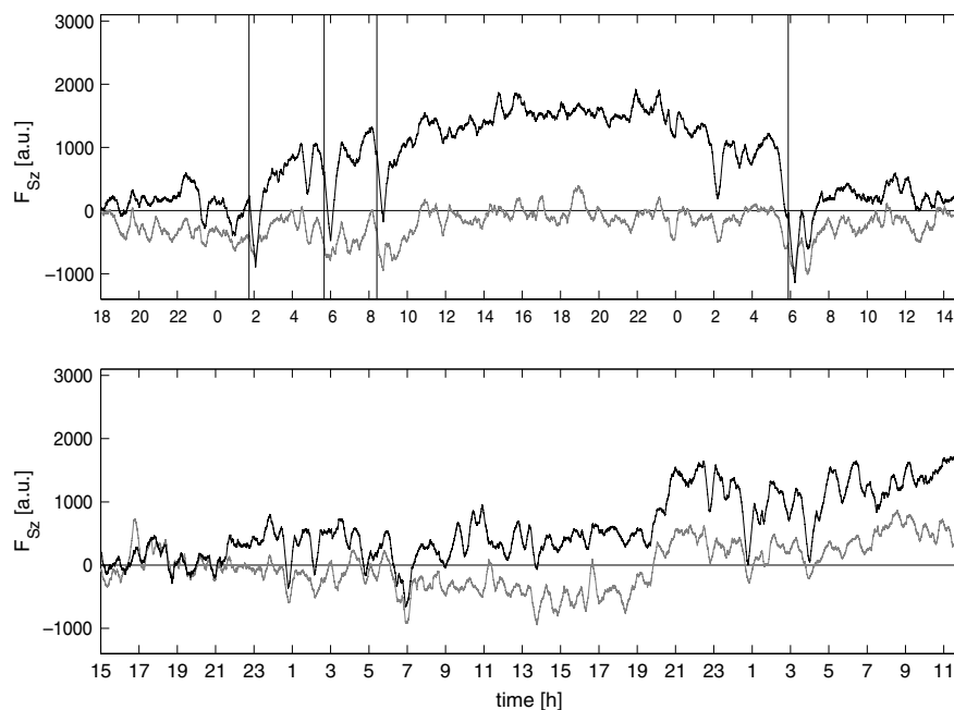
Fig. 6. Time continuous course of feature F_{Sz}(t) over 90 h calculated on invasive (black) and scalp (gray) EEG recordings of patient 01. Electroencephalographic seizure onsets are marked by vertical lines.
