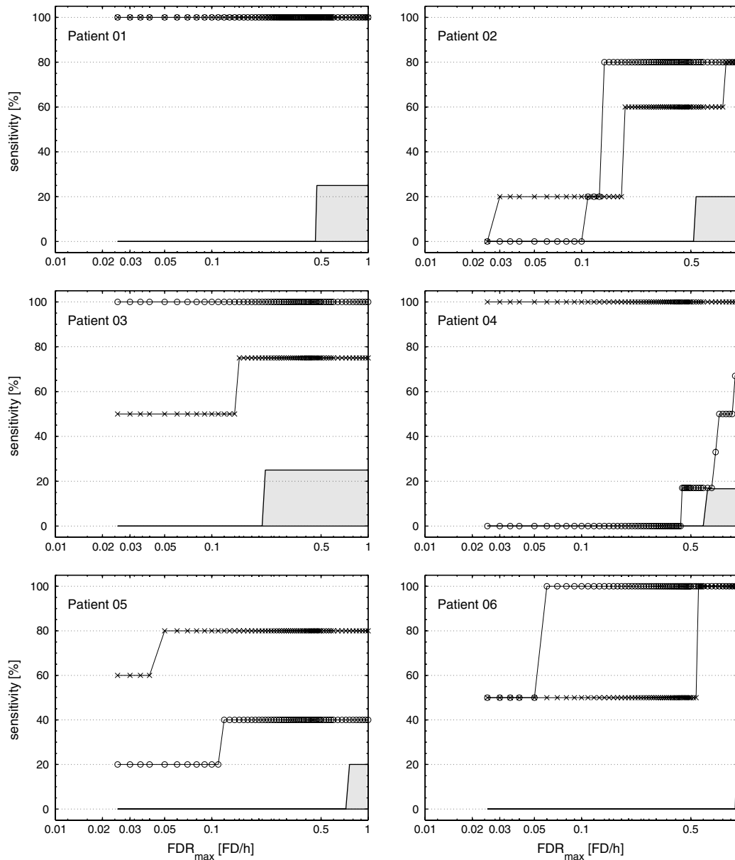
Fig. 4. Sensitivity of the investigated detection method in dependence on the maximum false detection rate for each patient. Different graphs result from the scalp EEG ( \times ) and from invasive EEG ( \circ ) recordings. Gray shaded areas mark non-significant regions \sigma_{\text{rand},0.05} of sensitivity.
