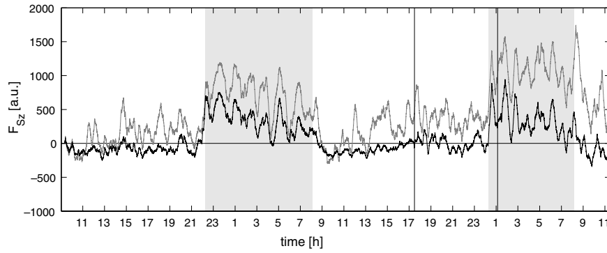
Fig. 7. Features F_{Sz}(t) of patient 06 calculated from invasive EEG (black) and scalp EEG (gray) data showing a circadian rhythm. Electroencephalographic seizure onsets are marked by vertical lines. Shaded regions mark times at which the patient was sleeping.
