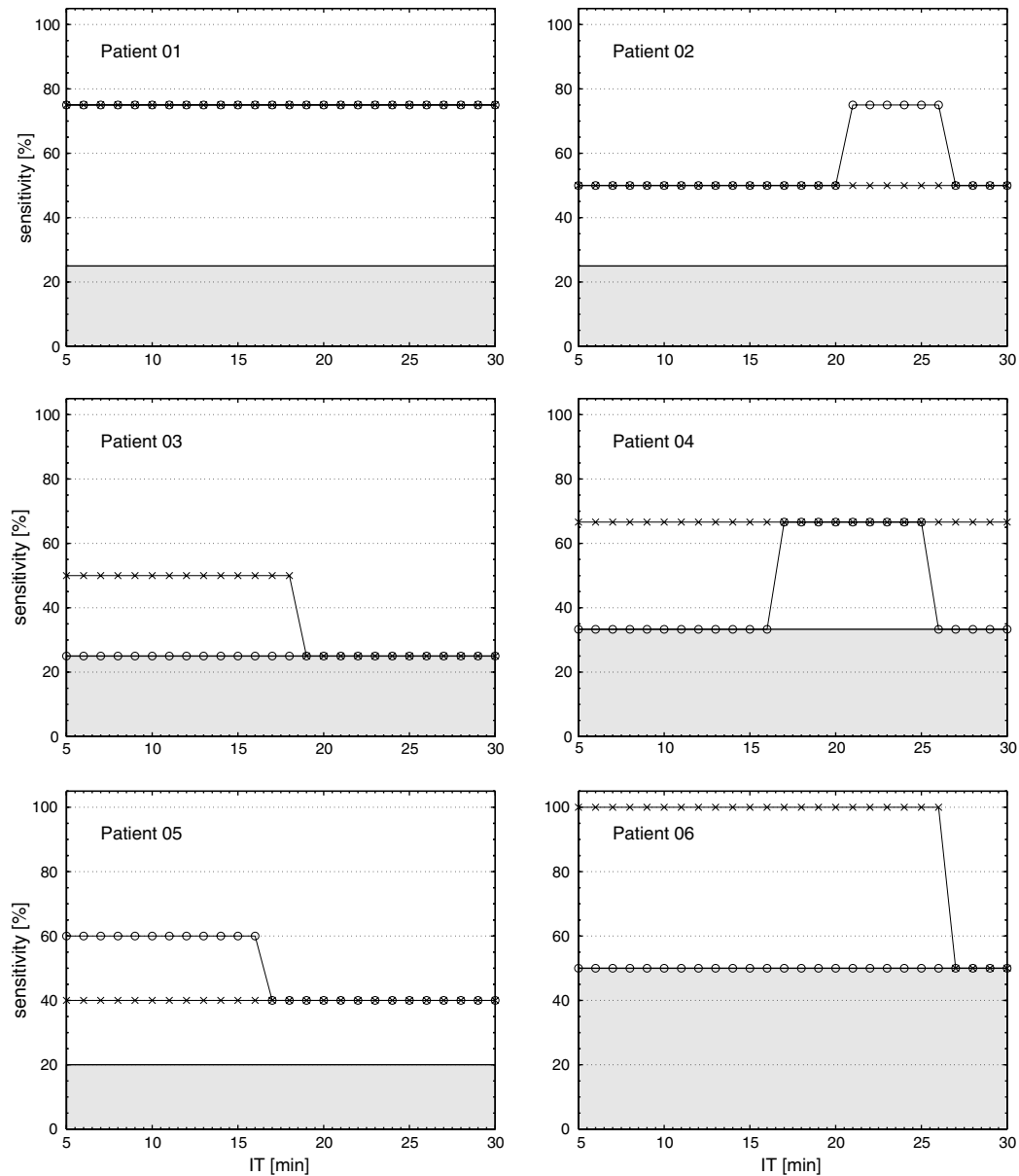
Fig. 10. Dependency of sensitivity on the intervention time IT with fixed SOP = 30 min and FPR_{\max} = 0.15 FP/h. Different graphs result from scalp EEG (x) and from invasive EEG (O) recordings. Gray shaded areas mark non-significant regions of a 5% significance level of a random predictor.
