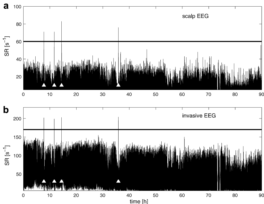
Fig. 1. Detection of seizures: Time course of the spiking rate SR over 90 h calculated on scalp (a) and invasive (b) EEG recordings from patient 01. Electroencephalographic seizure onsets are marked by triangles. An exemplary threshold for SR is given by a horizontal line. At the seizure onsets the spiking rate increases significantly. Threshold crossings coincide with marked seizures in (a) and (b), i.e. all four seizures are detected using scalp as well as invasive EEG data.
