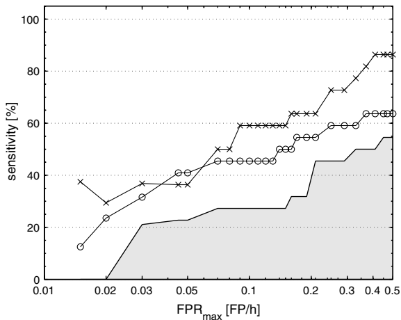
Fig. 9. Comparison between averaged performances of the seizure prediction method obtained from scalp ( \times ) and invasive ( \circ ) EEG recordings and averaged critical values of a random predictor (gray area) in dependence on the false prediction rate FPR_{max} . The parameter IT is set to 5 min and SOP to 30 min.
