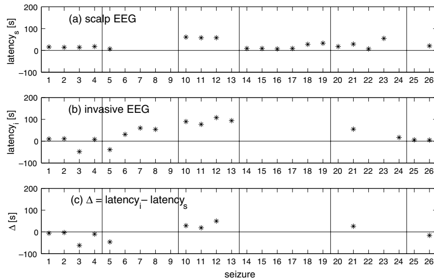
Fig. 3. Latencies of threshold crossing times of the spiking rate from scalp EEG (a) and invasive EEG (b) with respect to the electrographic seizure onset for all investigated seizures of all patients. Negative values represent detection before electrographic seizure onset. The difference \Delta = \text{latency}_i - \text{latency}_s , between latencies from invasive and scalp EEG, is shown in (c). Negative values of \Delta represent an earlier detection from invasive EEG data and positive values an earlier detection from scalp EEG data, respectively. Vertical lines separate seizures of different patients.
